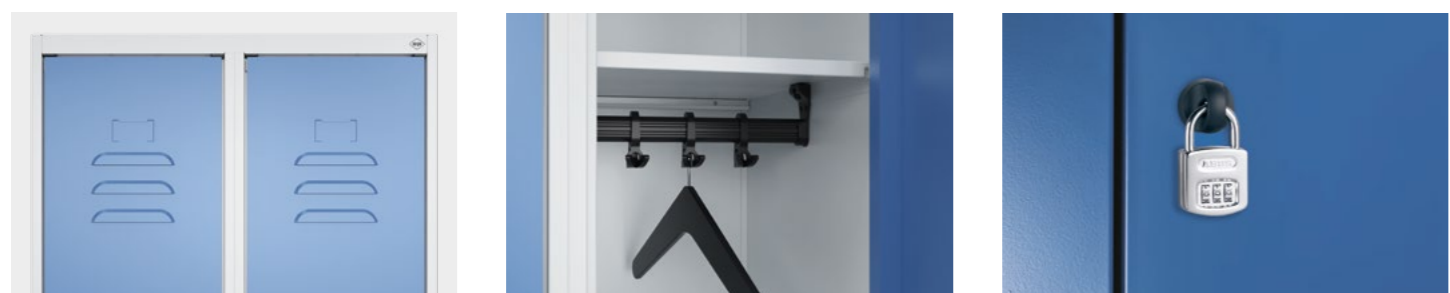
Classic vent slots with die-cut label holders Secure double sliding hooks with hanging option for hotel clothes hangers The picture shows the safety turning bolt. The series enables 34 different closing variants in total.
